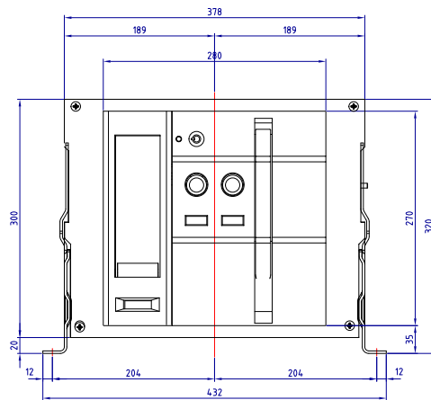
AS 2000/3200 3P Fixed ACB
