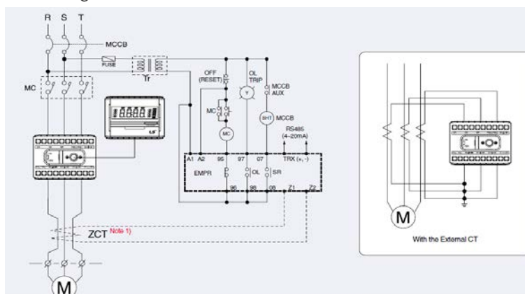
IMP Wiring Method
