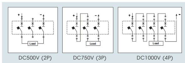
Exemplary circuit diagram
